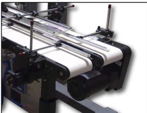
RLC250 Split Belt Orientation
