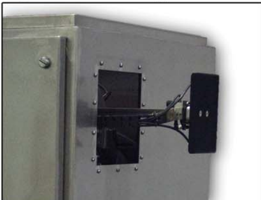
Optional Automated Application Door
